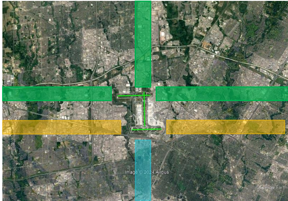
Typical use of Preferential Runway system
